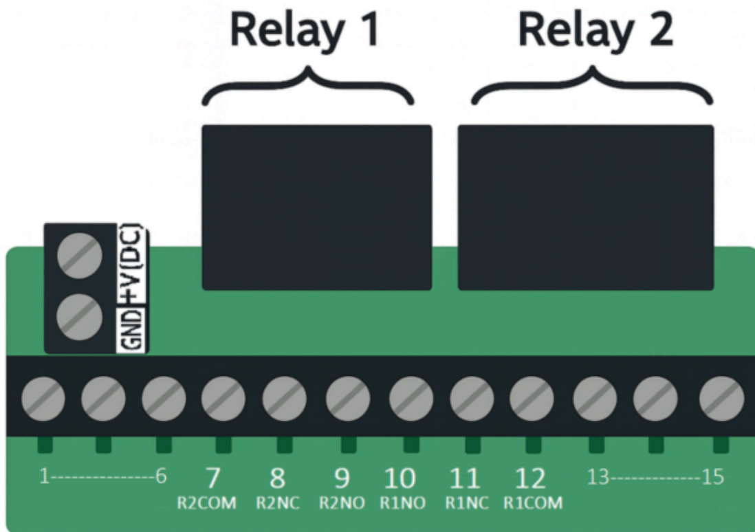
Simplified vector diagram of the relay block for user guidance
